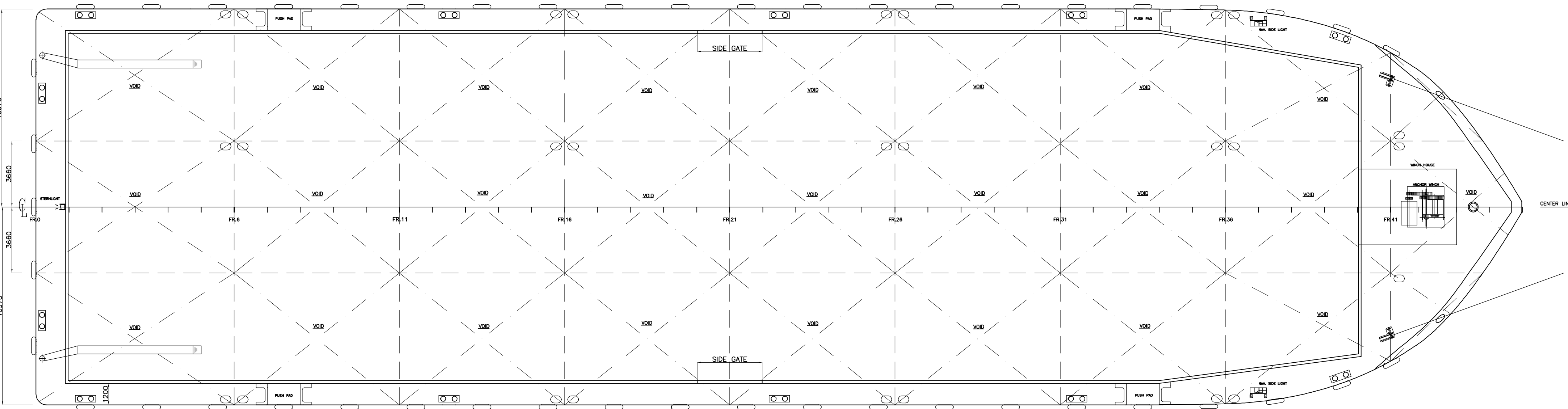
MAIN DECK PLAN
